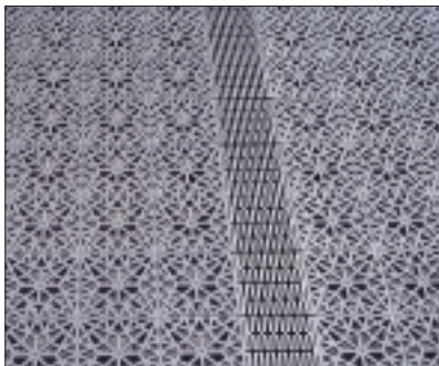
THE BERGO MARINE TILES with Expansiontiles in the middle. The Expansiontiles prevents the floor from expansion in varying temperatures.
